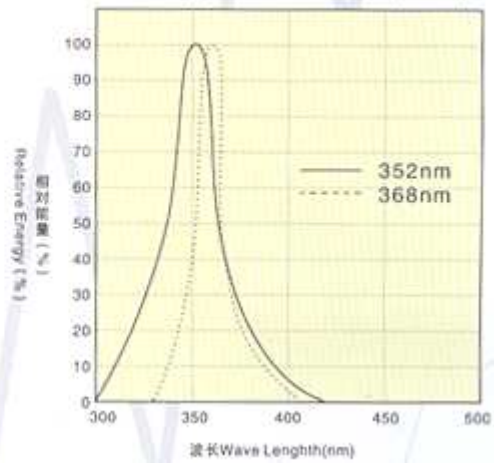
● 黑光蓝光灯 Blacklight Blue Lamp (BLB)
