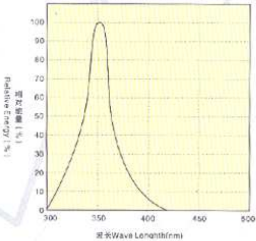
● 黑光灯 Blacklight Lamp (BL)
