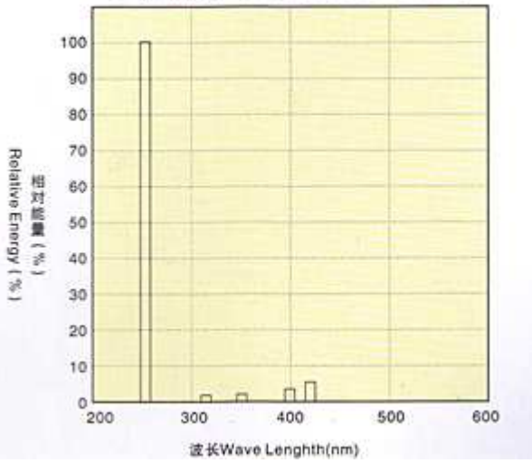
● 杀菌灯 Germicidal Lamp
